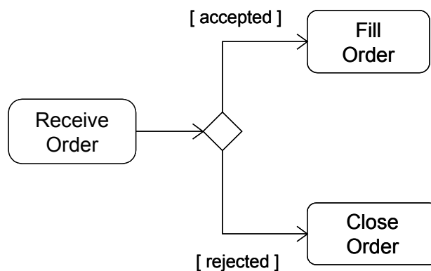
Figure 3: Decision Node
