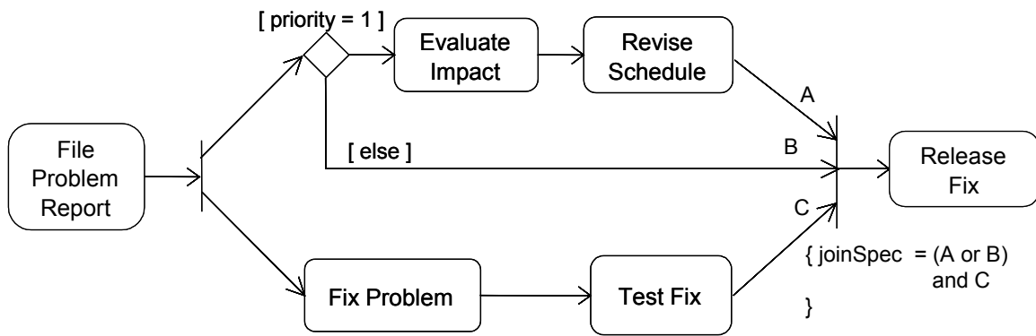
Figure 17: Join Specification
