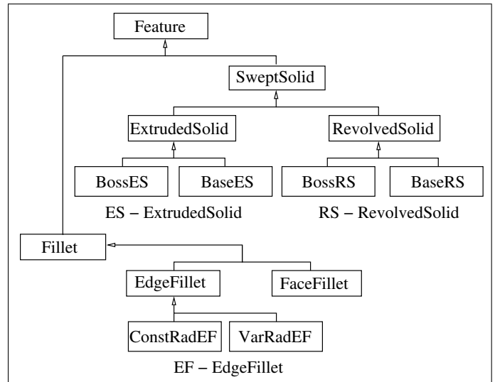
Figure 2. Partial taxonomy of features of example product(Fig. 1)
