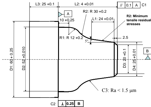
Fig. 3: Part design
