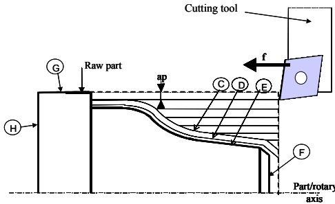
Fig. 4: Schematic process plan
