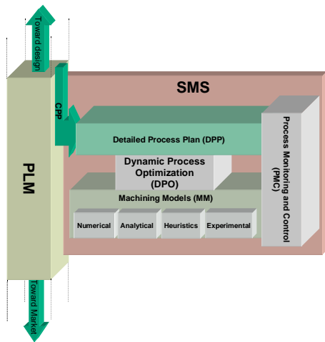
Fig. 2: SMS components
