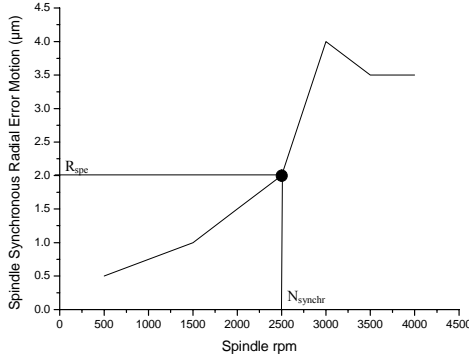
Fig. 8: Spindle Synchronous Radial Error Motion as a function of spindle speed
