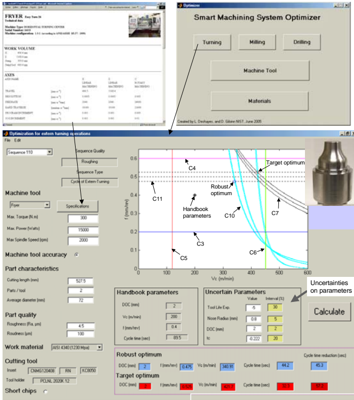
Fig. 5: Robust optimizer user interface
