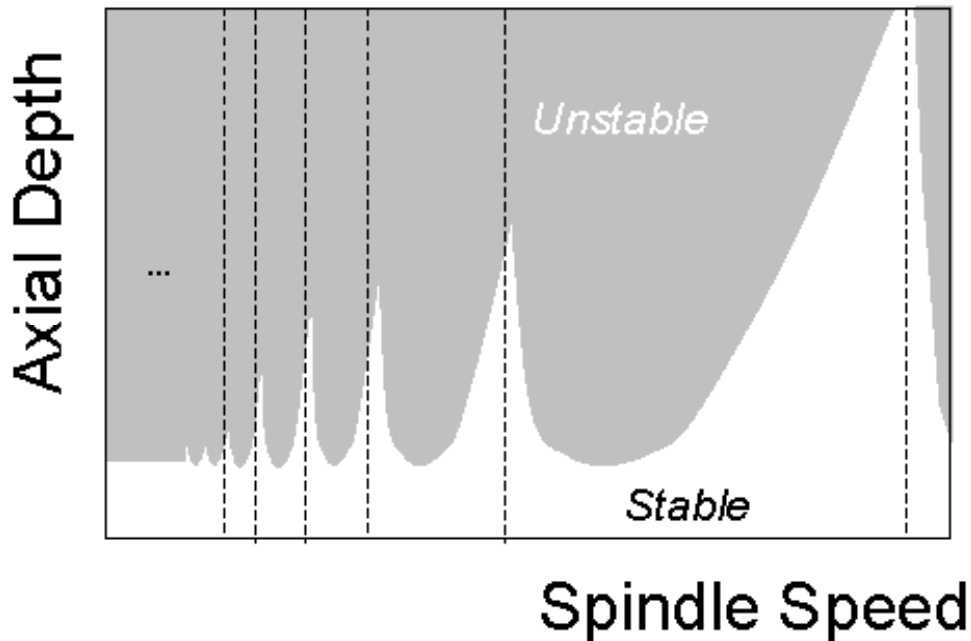
Figure 1: Stability lobe diagram
